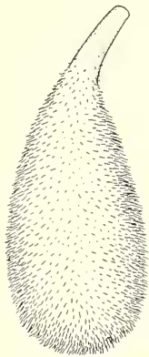
TEXT-FIG. 1. Suggested reconstruction of Schopfitheca boulayoides ; \times 2 .
